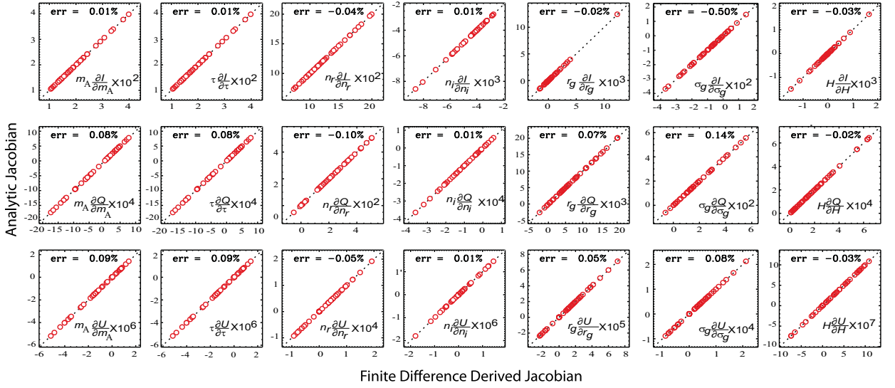
Fig. 5. Intercomparison of Jacobians ( \partial\xi/\partial \ln x ) calculated with UNL-VRM using the analytical method (y-axis) and those computed from UNL-VRM using finite difference estimates (x-axis). Here S is one of the Stokes parameters: I (top row), Q (middle row), and U (last row). x is one of 7 parameters associated with fine-mode aerosols - these parameters are the mass M (first column from the right), optical depth \tau (2nd column), real part m_r (3rd column) and imaginary part m_i (4th column) of the refractive index, geometric radius r_g (5th column) and geometric standard deviation \sigma_g (6th column) of the lognormal size distribution, as well as the aerosol peak height H (7th column). Note, the calculation is done for an atmosphere containing both fine (sulfate) and coarse (dust) mode aerosols as described in Hess et al. [63].
