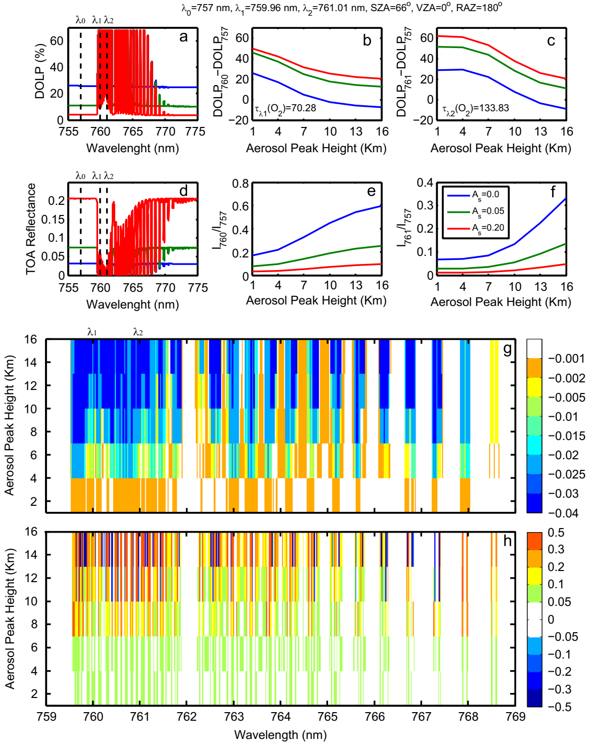
Fig. 7. (a) Simulated DOLP, and (d) normalized radiances (i.e. assuming incoming solar irradiance of unity, bottom row) in the spectral range of 755–775 nm at the top-of-atmosphere for 3 surface reflectances ( A_s ) respectively of 0 (blue line), 0.05 (green line), and 0.2 (red line). The aerosol altitude is set at 7 km, and aerosols are assumed spherical with lognormal size distribution having r_g = 0.5 \mu\text{m} and \sigma_g = 0.2 \mu\text{m} , and with refractive index 1.53–0.008i. Plots (b) and (c) respectively show the changes of DOLP at two \text{O}_2 A band wavelengths ( \lambda_1 and \lambda_2 ) with respect to the DOLP value in the continuum ( \lambda_0 ). Plots (e) and (f) are respectively the same as (b) and (c), but for the change of reflectance. Plot (g) shows the moving averages of Jacobians of DOLP with respect to relative change of aerosol height ( \partial\text{DOLP}/\partial\ln H ), while plot (h) shows the moving averages of the differences of absolute values of normalized Jacobians between DOLP and I with respect to the relative change of height ( |\partial\ln\text{DOLP}/\partial\ln H| - |\partial\ln I/\partial\ln H| ). See text for details.
