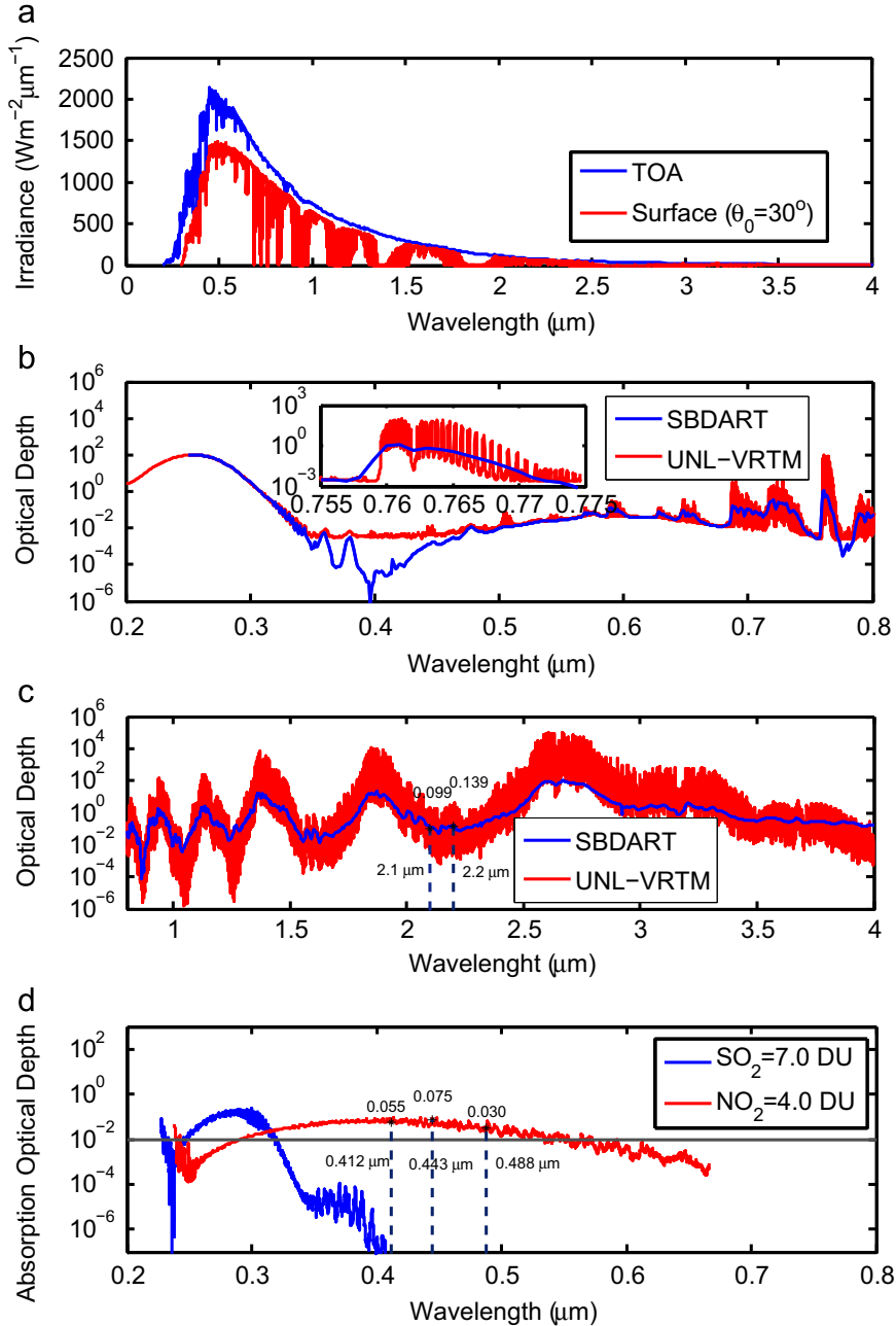
Fig. 2. (a) Downward solar spectral irradiance at the TOA and the surface for solar zenith angle of 30^\circ . (b) Total-atmosphere gas absorption optical depth in the range 0.2–0.8 \mu\text{m} . (c) Same as (b) but for 0.8–4 \mu\text{m} . (d) Optical depth of \text{SO}_2 and \text{NO}_2 in polluted cases. Also shown in (b) and (c) are the optical depth computed from Santa Barbara DISORT Atmospheric Radiative Transfer (SBDART) model [45]. The mid-latitude summer atmospheric profile is assumed (McClatchey et al. [62]).
