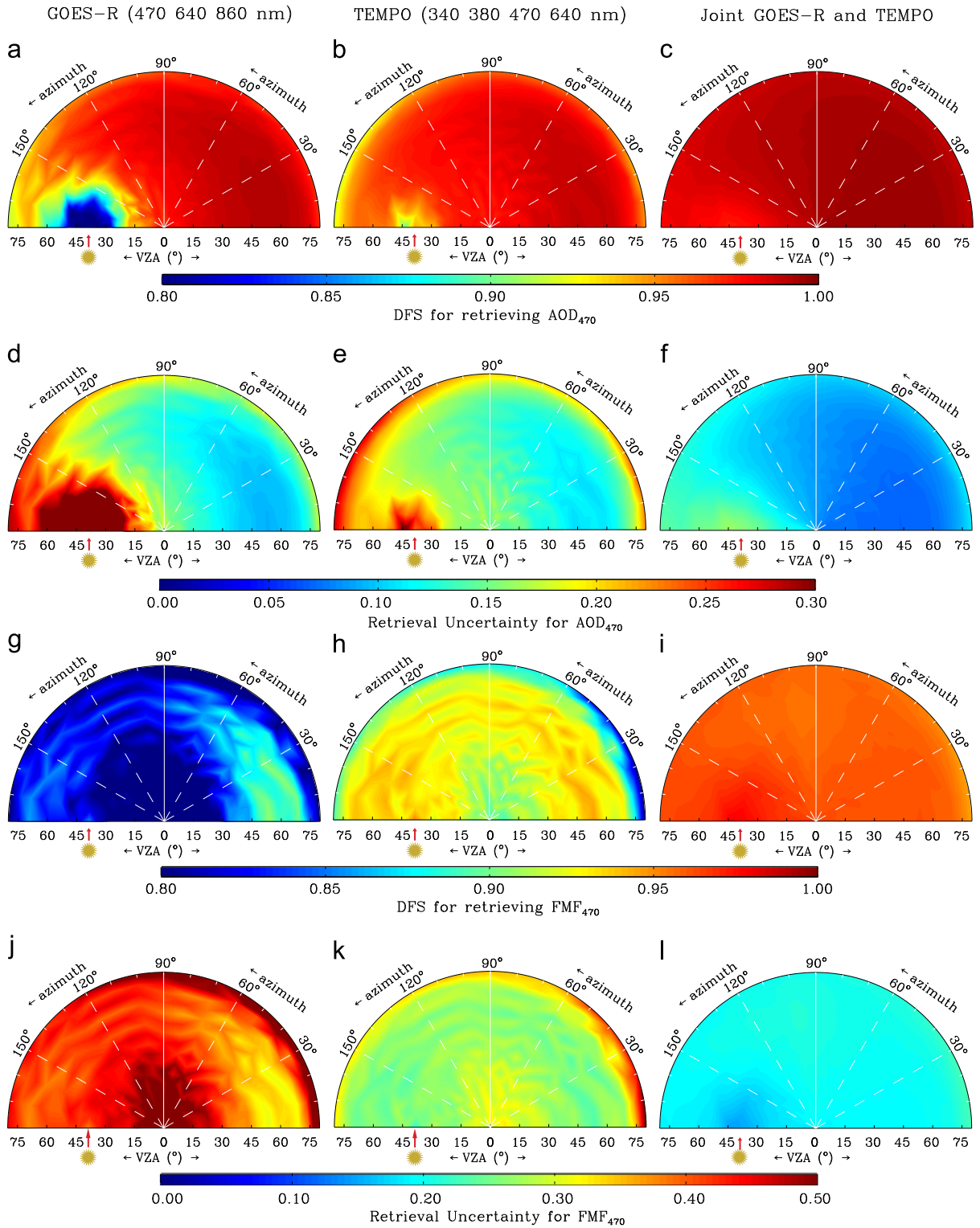
Fig. 10. Polar plots of Degree of Freedom for Signal (DFS) for the retrieval of the total aerosol optical depth at 470 nm ( AOD_{470} ) from: (a) GOES-R, (b) TEMPO, and (c) joint measurements of GOES-R and TEMPO. Plots (d)–(f) are retrieval uncertainties for AOD_{470} from these three sets of measurements, respectively. Plots (g)–(l) are similar to (a)–(f) but apply to the retrieval of 470 nm AOD fine-modal fraction ( FMF_{470} ). Note that the three atmospheric window channels from TEMPO are the ones used by AERONET to measure AOD . In each polar plot, the VZA is shown as the radius, while the polar angle represents the relative azimuth. The solar zenith angle is fixed at 40^\circ . Values for joint retrieval correspond to the VZA for GOES-R and averages for different sets of VZA for TEMPO. The two modes are for sulfate- and dust-like aerosols with optical depths of 0.78 and 0.28 respectively at 470 nm. An underlying grass surface is assumed, with MODIS-retrieved BRDF parameters.
