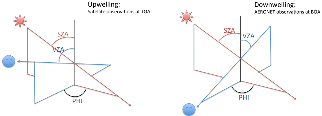
Figure 1: Illustration of UNL-VRTM geometry. SZA: solar zenith angle, VZA: viewing zenith angle, PHI: relative azimuth angle.
